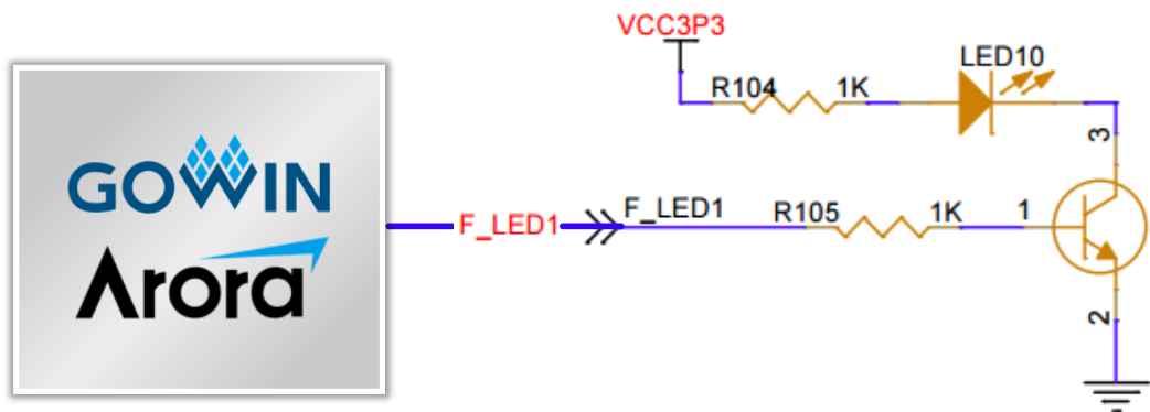
Figure 3-11 Connection Diagram of LED
