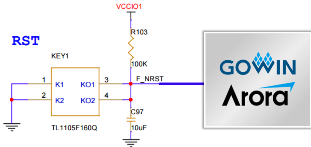
Figure 3-10 Connection Diagram of Key
