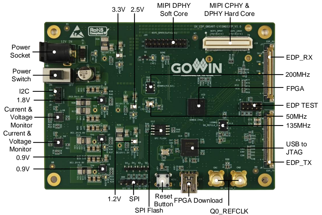
Figure 2-3 PCB Components
