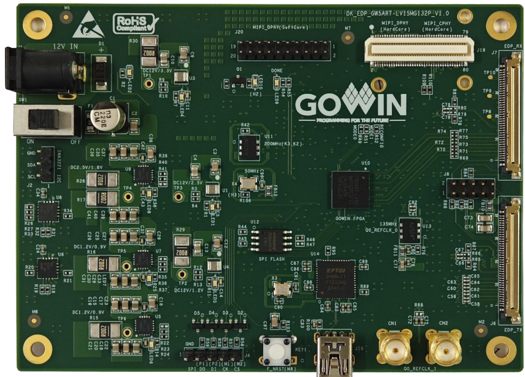
Figure 2-1 DK_EDP_GW5ART-LV15MG132P_V1.0 Development Board
