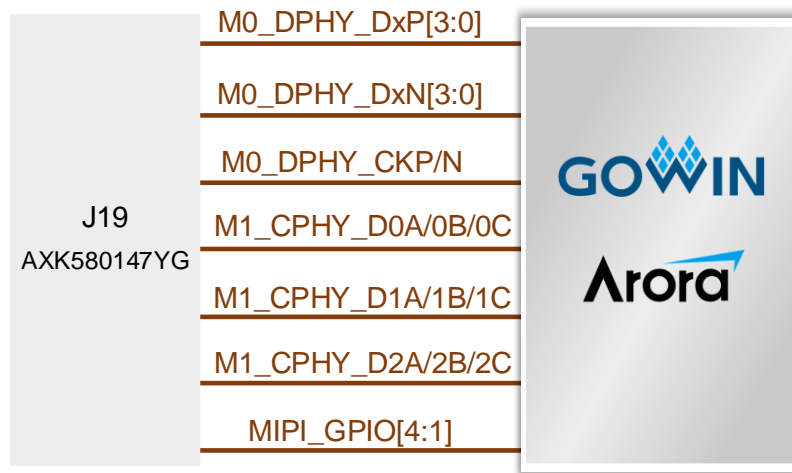
Figure 3-5 Connection Diagram of MIPI CPHY &amp; DPHY Hard Core Interfaces
